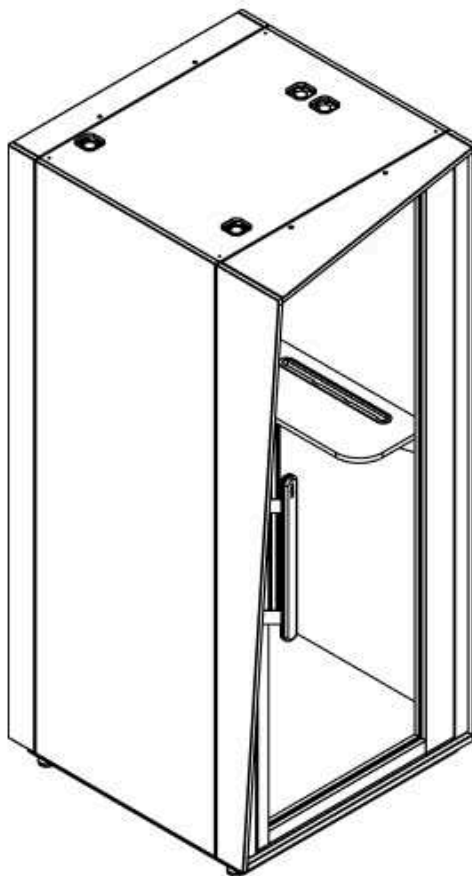
BMG-RH Phonebooth With kink. Right-hand opening.
