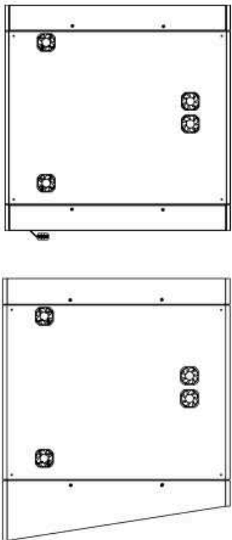
Plan view 4 x ventilation fans. Top: no kink Bottom: with kink
